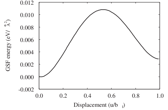
FIG. 9. GSF energy for copper on the (11 \bar{1} ) plane along the [\bar{2}1\bar{1}] direction. The displacement is normalized by |b_l|=a/\sqrt{6} , which is the magnitude of Burgers vector of a Shockley partial dislocation.
