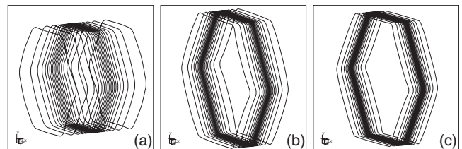
FIG. 4. Core structure of self-interstitial loops containing (a) 91, (b) 397, and (c) 919 SIAs in iron. Each line represents one infinitesimal dislocation loop and is also considered as an equidisplacement contour line incremented by b/20 ( \sim 0.014 \text{ nm} ).
