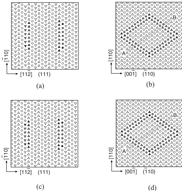
FIG. 11. Atomic arrangements of the core structure of a cluster containing 100 SIAs in copper obtained by MD calculations using the Mishin potential (a and b), compared with those obtained by the present method (c and d). The colors are based on the central symmetry technique; gray atoms form the SF, while black atoms surround the partial dislocation core. The atomic positions are projected on the (111) plane (a and c) and the \bar{1}10 plane (b and d).
