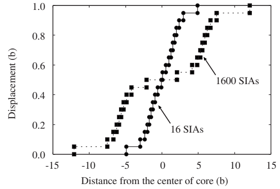
FIG. 12. Displacement distribution of SIA dislocation loop cores in copper for a small cluster containing 16 SIAs and for a large cluster containing 1600 SIAs.
