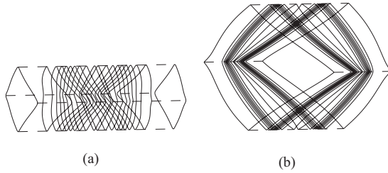
FIG. 10. Core structure of an SIA cluster modeled as a rhombus-shaped edge dislocation loop in copper containing (a) 16 and (b) 400 SIAs. Each line represents one infinitesimal dislocation loop and is also considered as an equidisplacement contour line incremented by b/20 ( \sim 0.006 nm).
